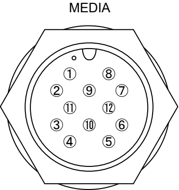
MEDIA cable: CFQ-7517 (optional)
