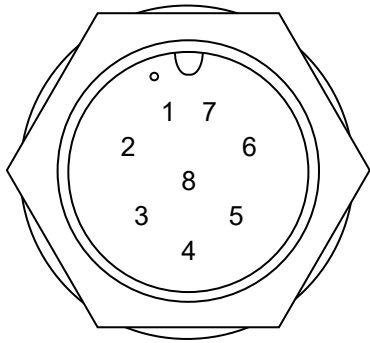
TRANSDUCER
